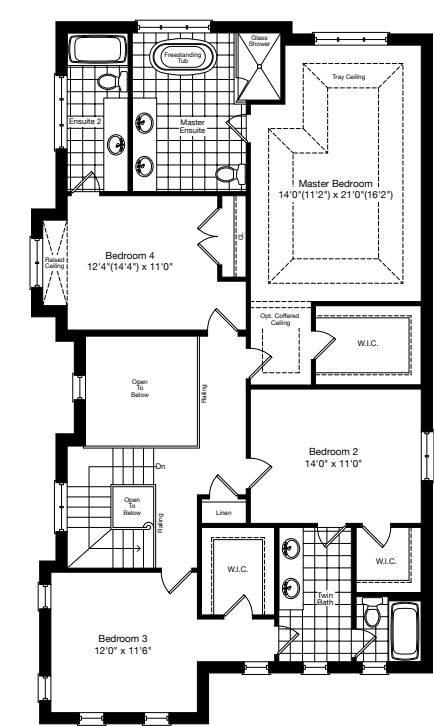
SECOND FLOOR ELEV. B
