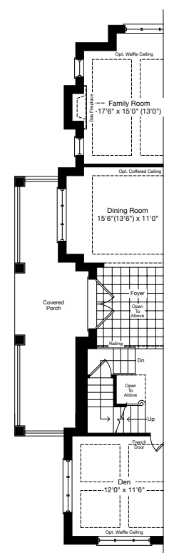
PARTIAL MAIN FLOOR ELEV. B
