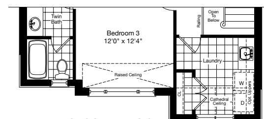
PARTIAL SECOND FLOOR ELEV. C
