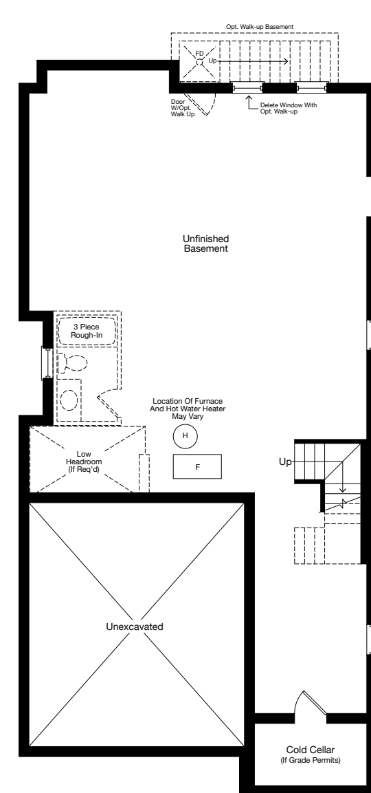
BASEMENT ELEV. A, B & C
