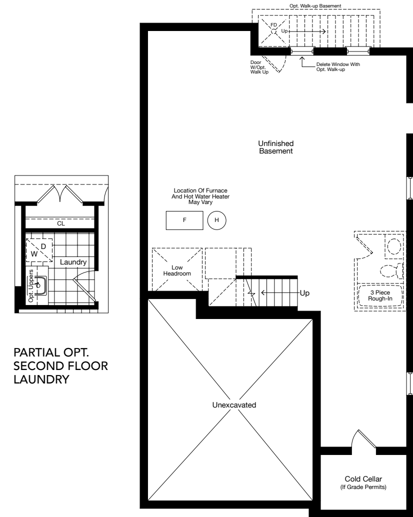
BASEMENT ELEV. A
