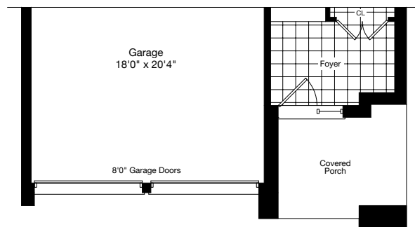
PARTIAL MAIN FLOOR ELEV. C
