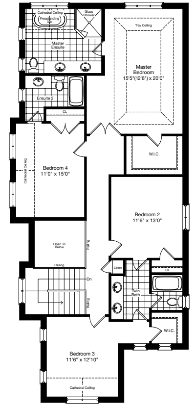
SECOND FLOOR ELEV. B
