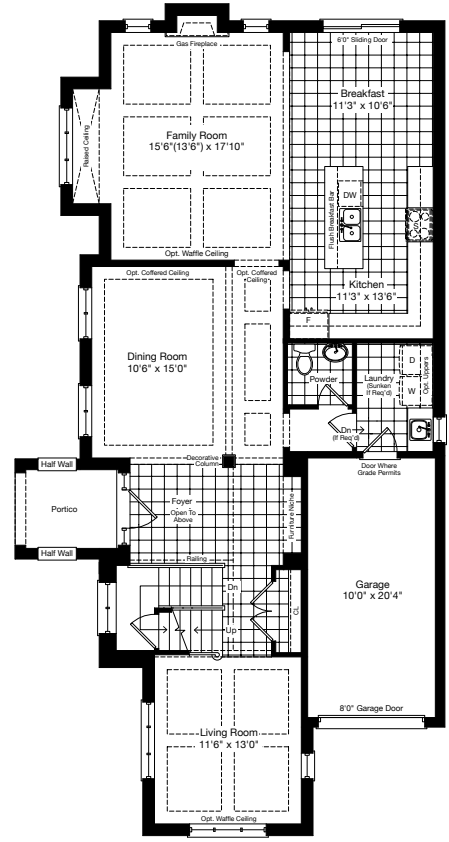
MAIN FLOOR ELEV. B
