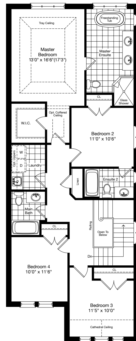
OPT. SECOND FLOOR ELEV. A
