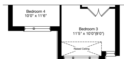
PARTIAL SECOND FLOOR ELEV. C
