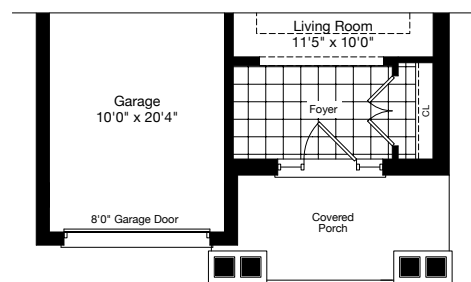
PARTIAL MAIN FLOOR ELEV. B
