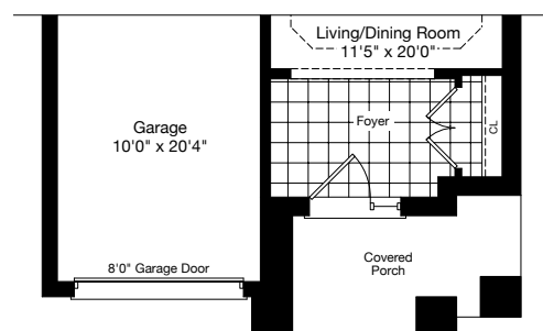
PARTIAL MAIN FLOOR ELEV. C
