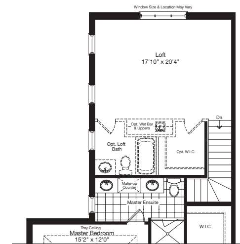
PART. OPT. SECOND FLOOR ELEV. C1 W/LOFT
