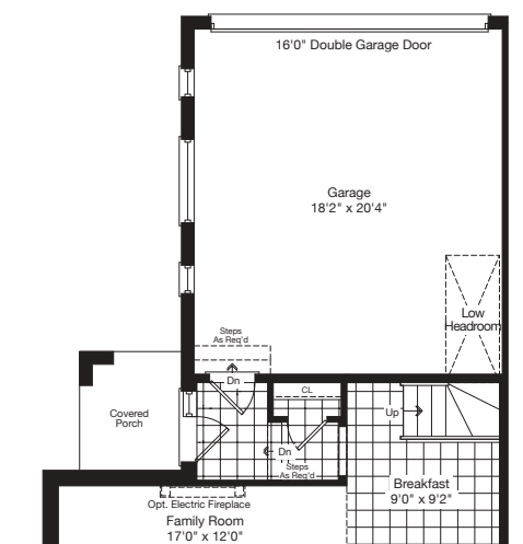
PART. OPT. MAIN FLOOR ELEV. C2 W/LOFT
