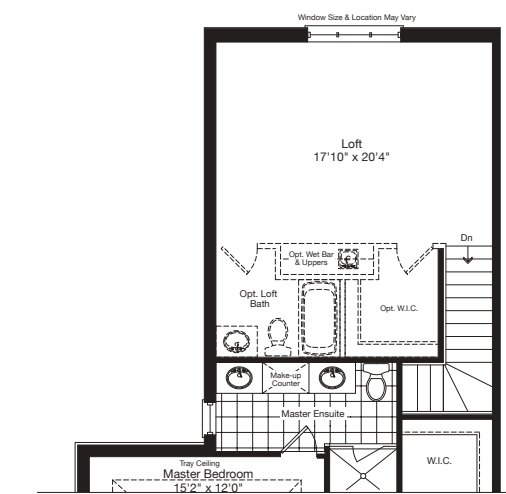
PART. OPT. SECOND FLOOR ELEV. C2 W/LOFT
