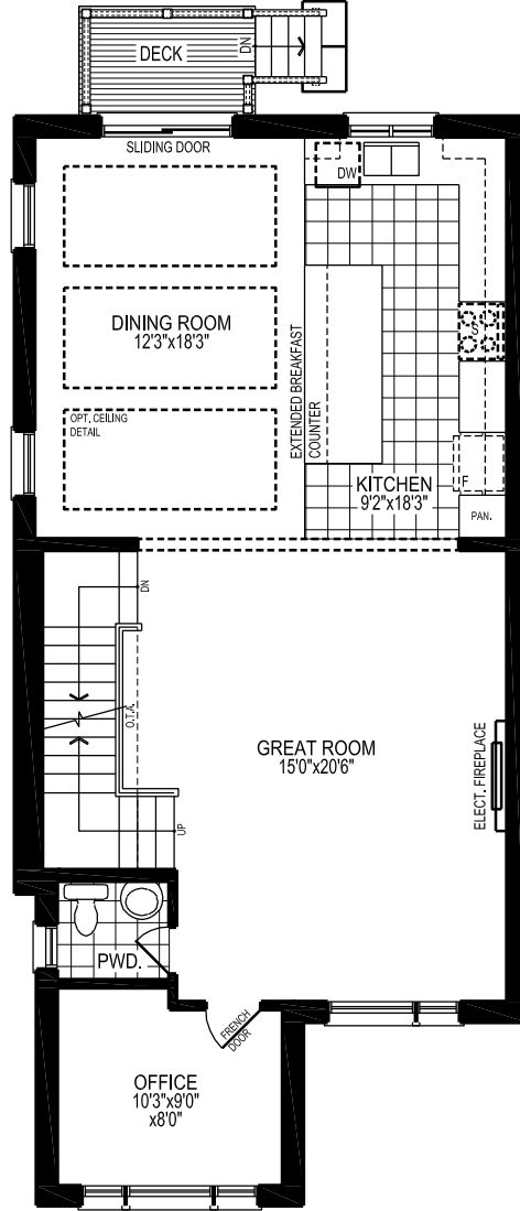
MAIN FLOOR PLAN, EL.'B'
