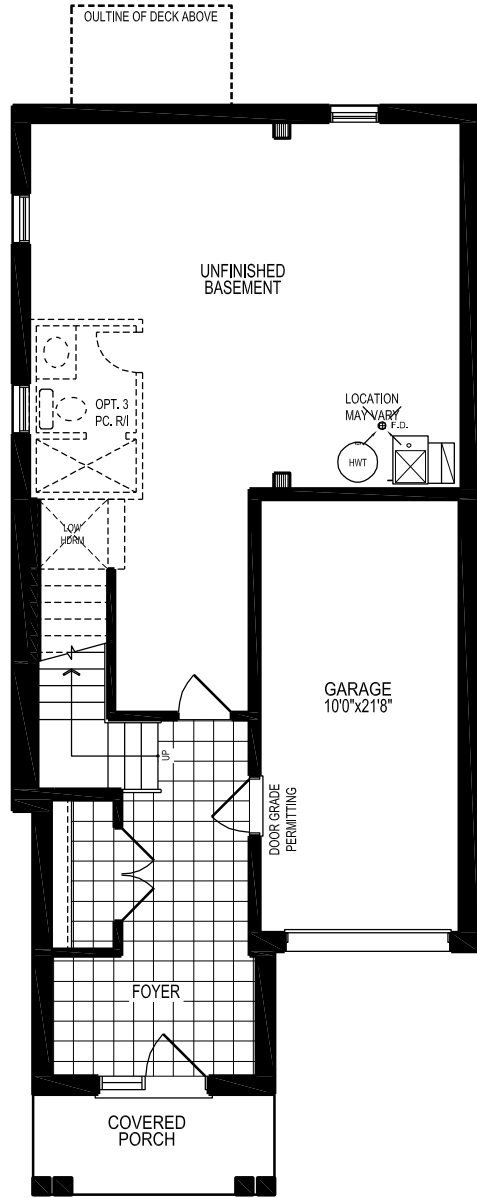
BASEMENT FLOOR PLAN, EL.'B'
