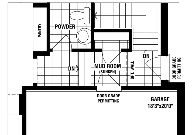
PARTIAL MAIN FLOOR WITH OPTIONAL SERVICE STAIRS (ELEVATION 'B' & 'C' SIMILAR)
