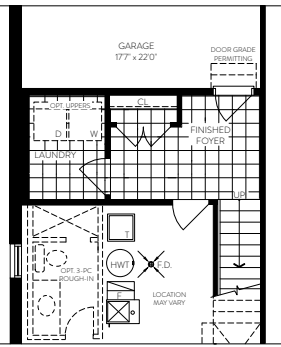
PART. BASEMENT FLOOR FOR 4 BEDROOM PLAN
