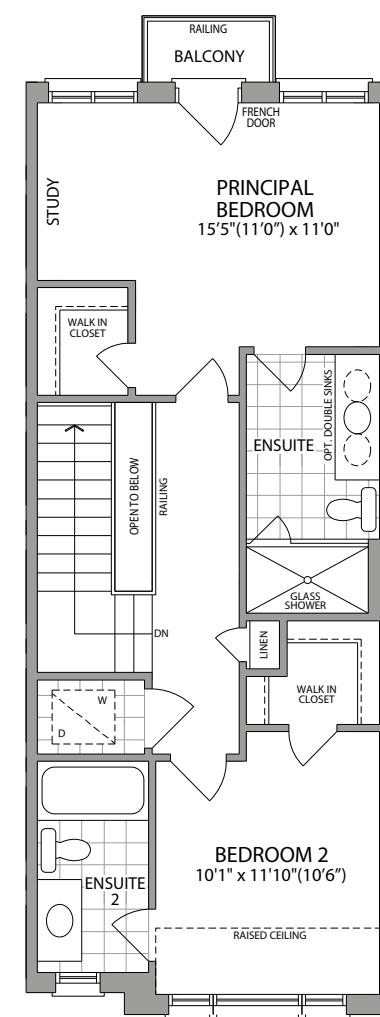
THIRD FLOOR ELEV. C1
