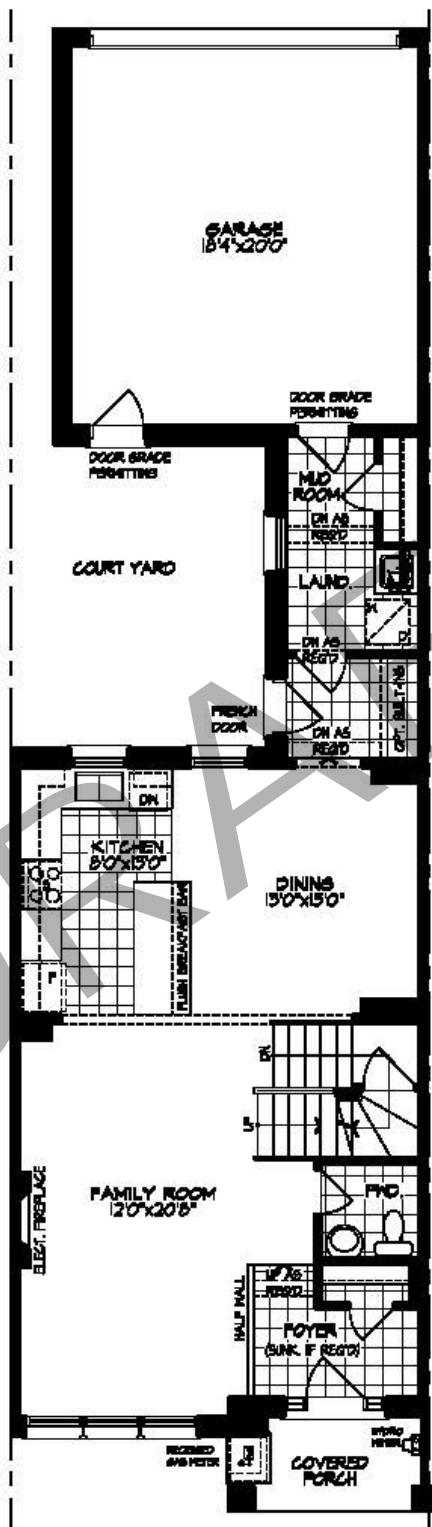
MAIN FLOOR PLAN, EL. 'C'
