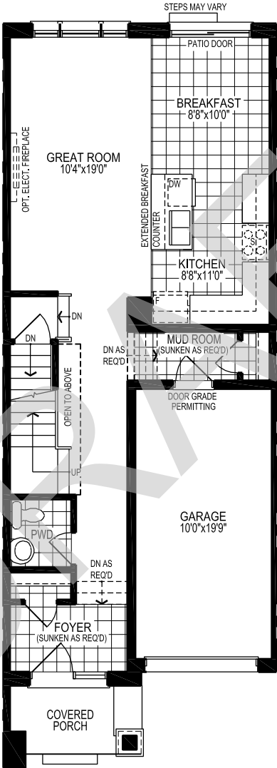
GROUND FLOOR PLAN, EL. 'C'
