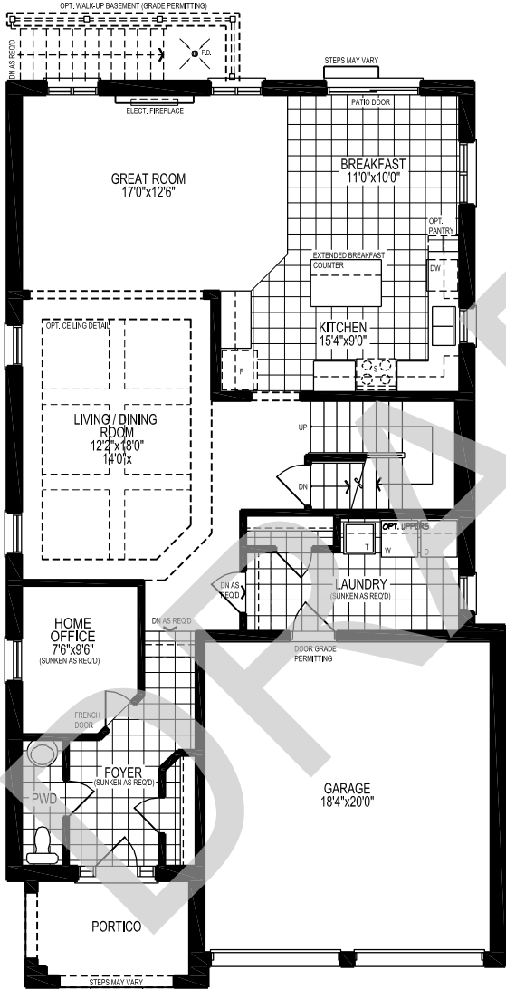
GROUND FLOOR PLAN, EL. 'C'
