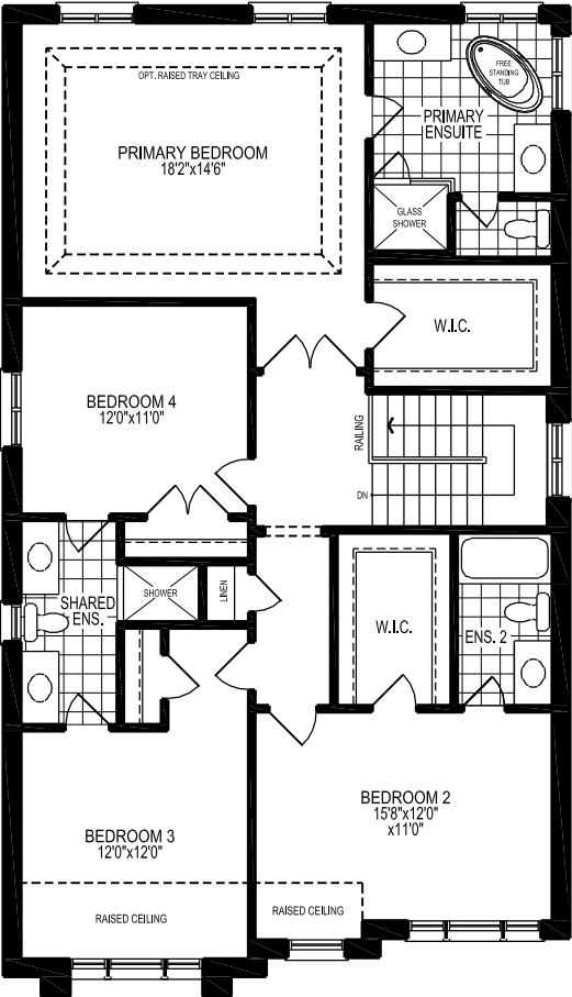
SECOND FLOOR PLAN, EL. 'C'
