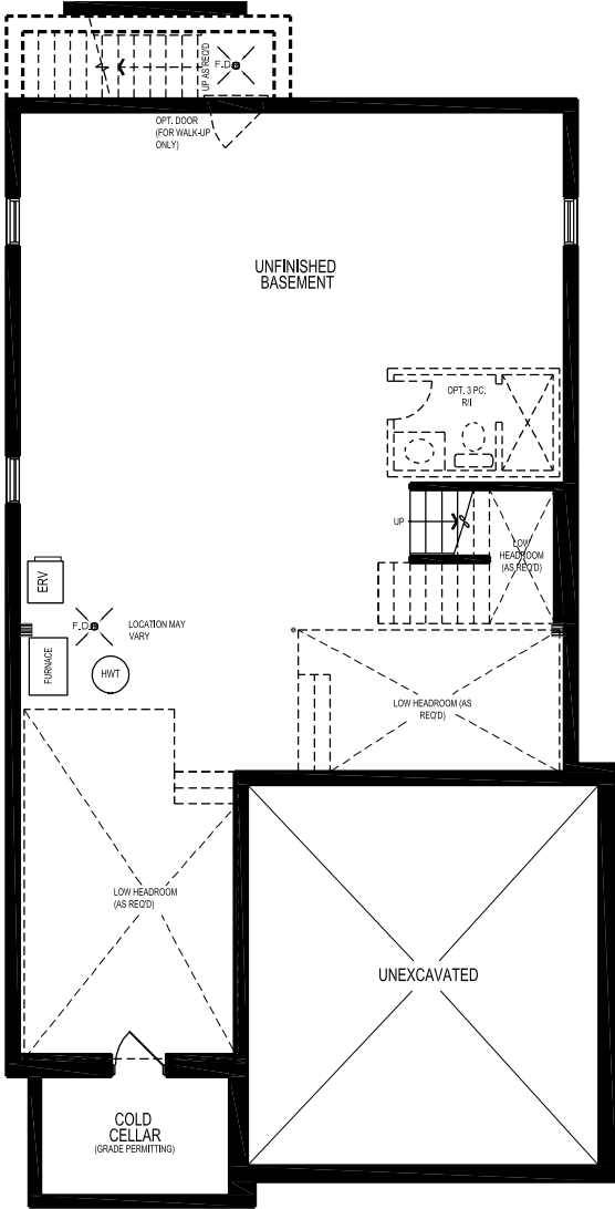
BASEMENT FLOOR PLAN, EL. 'C'
