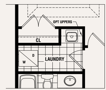
PARTIAL OPT. SECOND FLOOR LAUNDRY W/ STACKABLE WASHER AND DRYER ELEV. 'A-1', 'A-2', 'B-1' & 'B-2'
