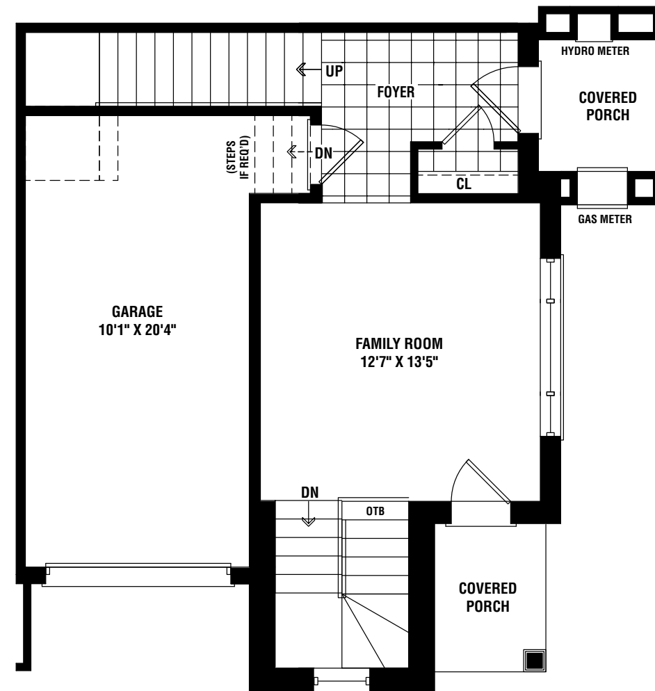
GROUND FLOOR ELEV. 'C1'
