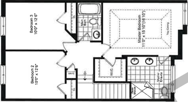
SECOND FLOOR ELEV. C1
