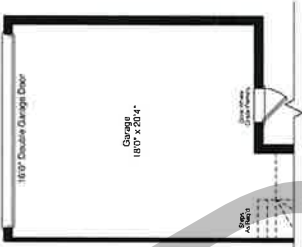
PART. OPT. MAIN FLOOR ELEV. C1 & C2 W/DOUBLE CAR GARAGE
