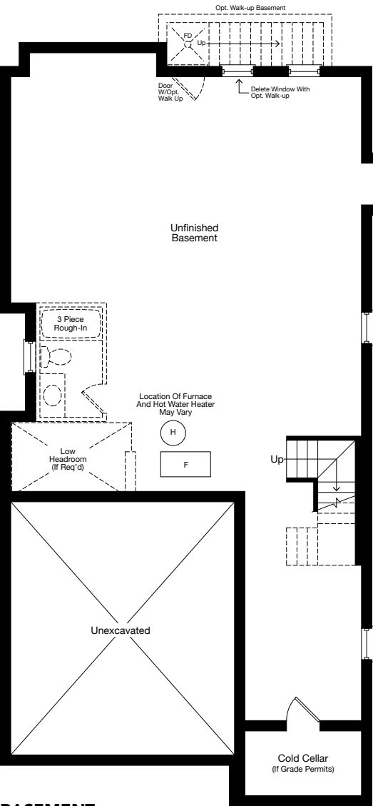
BASEMENT ELEV. A, B & C
