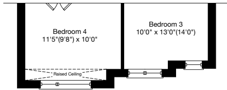
OPT. PARTIAL SECOND FLOOR ELEV. C
