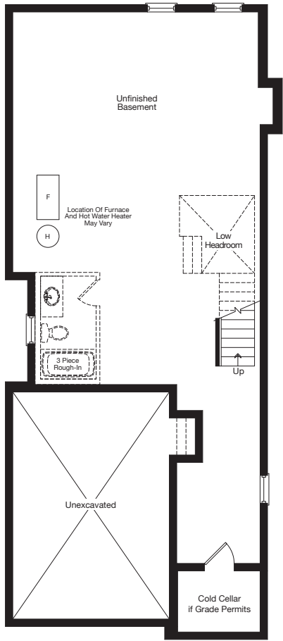
BASEMENT ELEV. A & B
