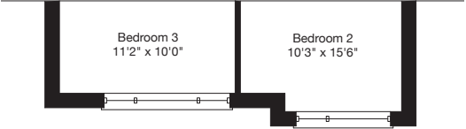
PARTIAL SECOND FLOOR ELEV. C
