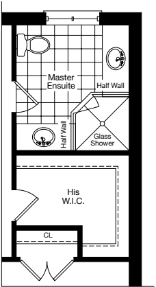
PARTIAL OPT. SECOND FLOOR MASTER ENSUITE LAYOUT
