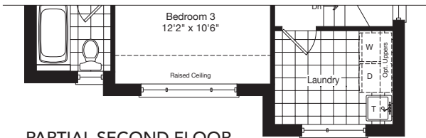
PARTIAL SECOND FLOOR ELEV. C
