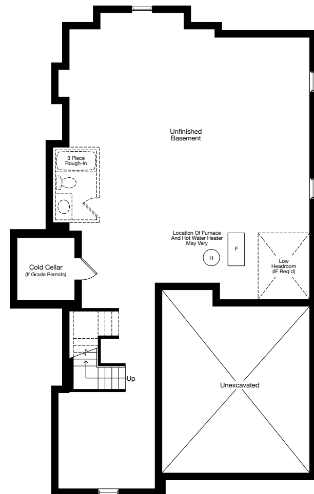
BASEMENT ELEV. A
