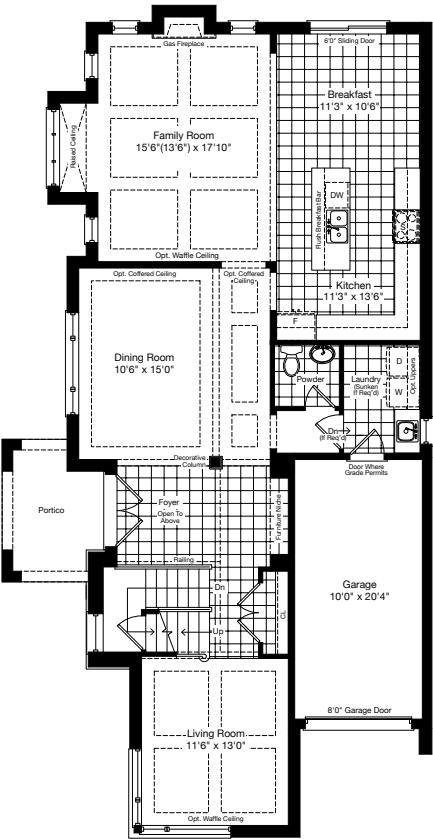
MAIN FLOOR ELEV. C
