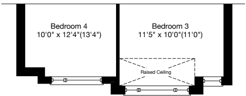
PARTIAL SECOND FLOOR ELEV. C
