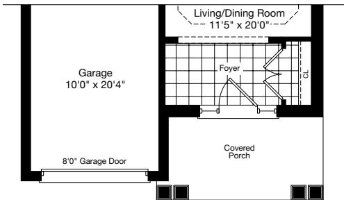
PARTIAL MAIN FLOOR ELEV. B
