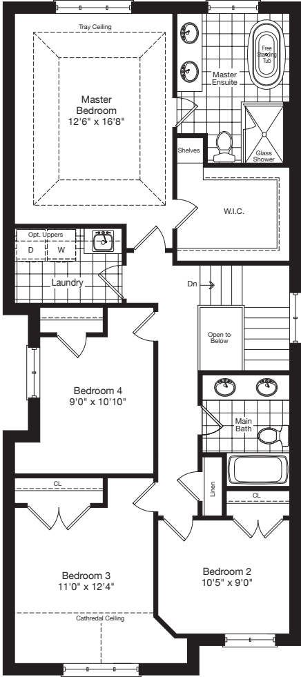
OPT. SECOND FLOOR ELEV. A
