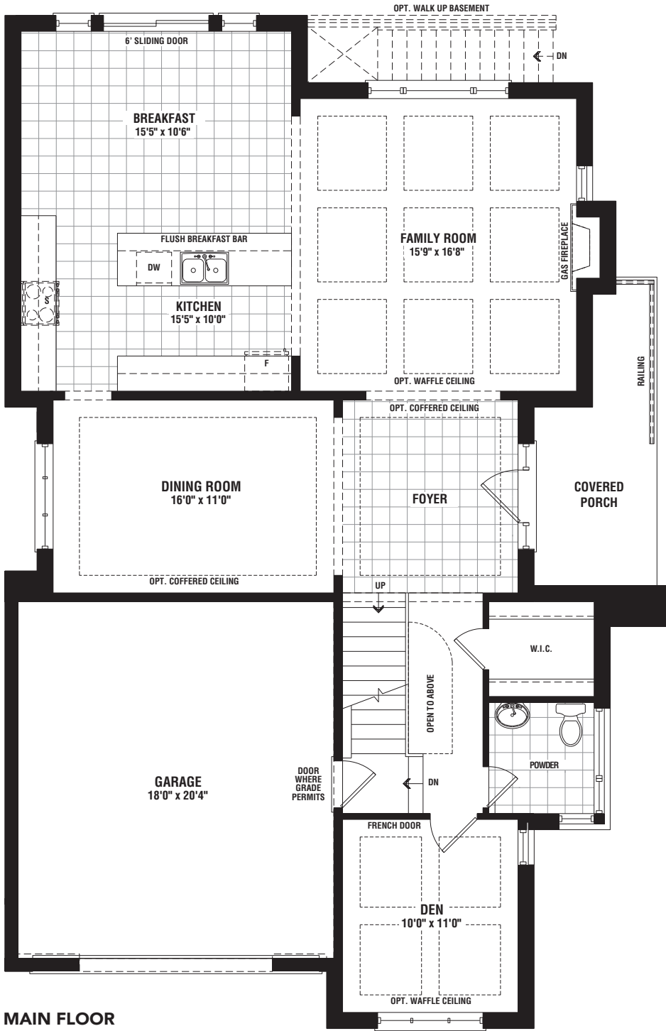
MAIN FLOOR ELEV. C1
