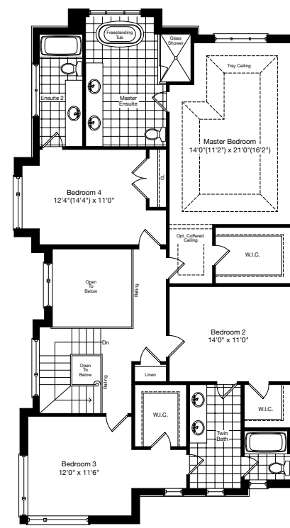
SECOND FLOOR ELEV. C
